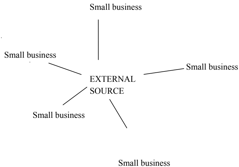
Figure 4.1 Centre-Periphery Model
