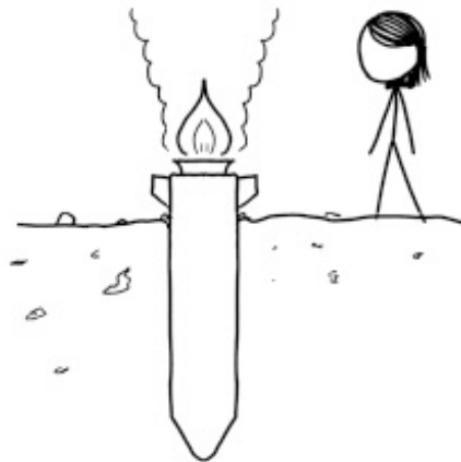
Geysir
